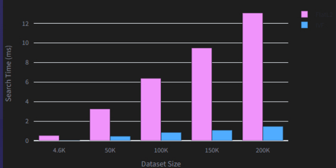
Search Time per Query: FlatL2 vs IVF
